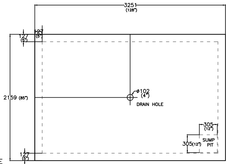
PADMOUNT FOUNDATION FLOOR
