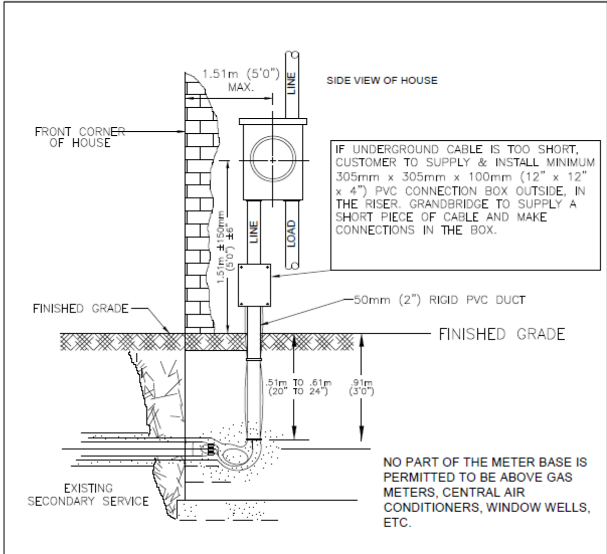
MS-004 Existing Overhead/Underground Service, Single-Phase 120/240V Meter Base Relocation (Inside to Outside) - Equipment Layout
